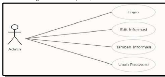
Gambar 1 Tampilan Use Case Diagram Admin
