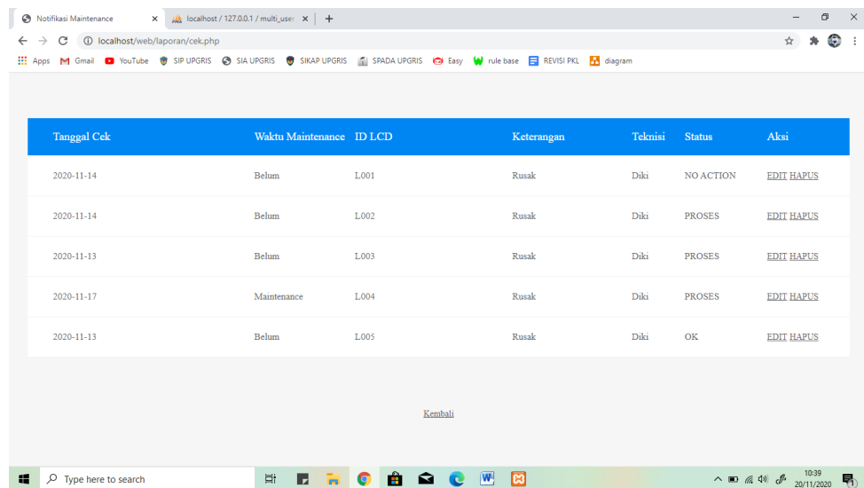
Gambar 4 Data Maintenance
